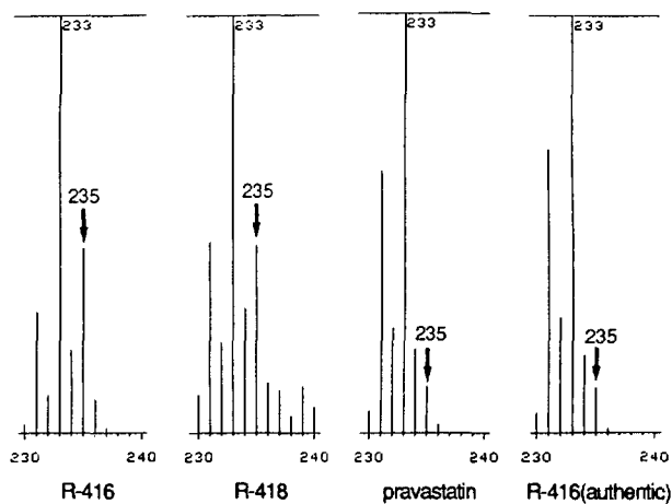
Figure 4. The part spectra(m/z 230-240) of R-416, R-418, and PV obtained after incubation of PV in the presence of H_2^{18}O and authentic R-416.
